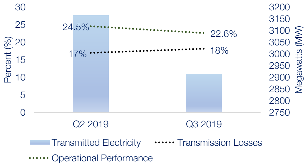
Figure 4: Transmitted Electricity, Transmission Losses and Operational Performance between April 2019 and September 2019. The monthly average was recorded for the period under review.
